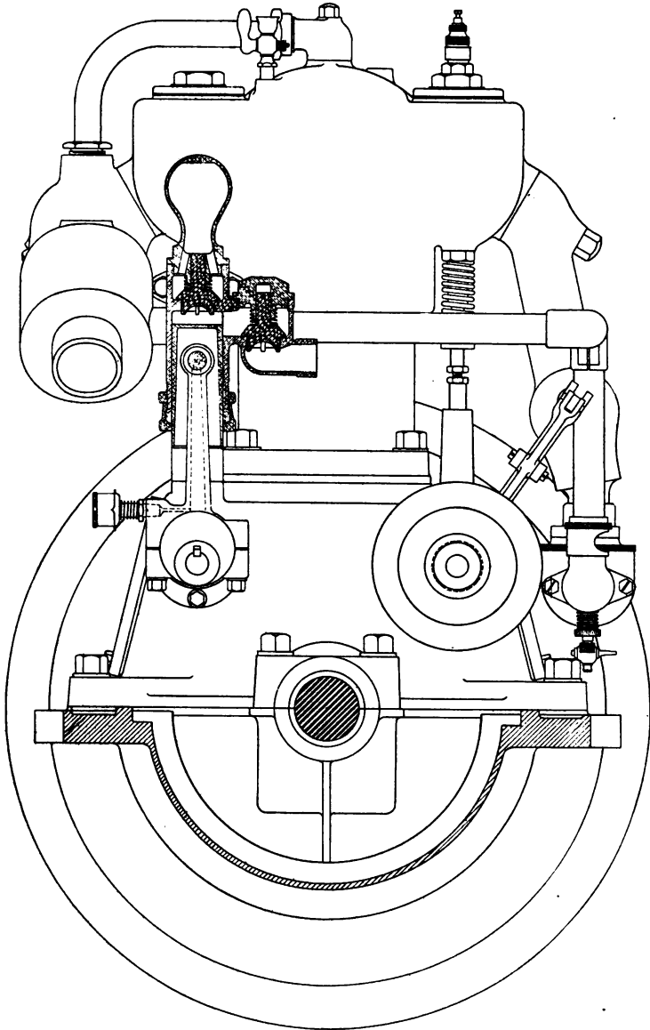
FIG. 64.—The Sterling Engine.
